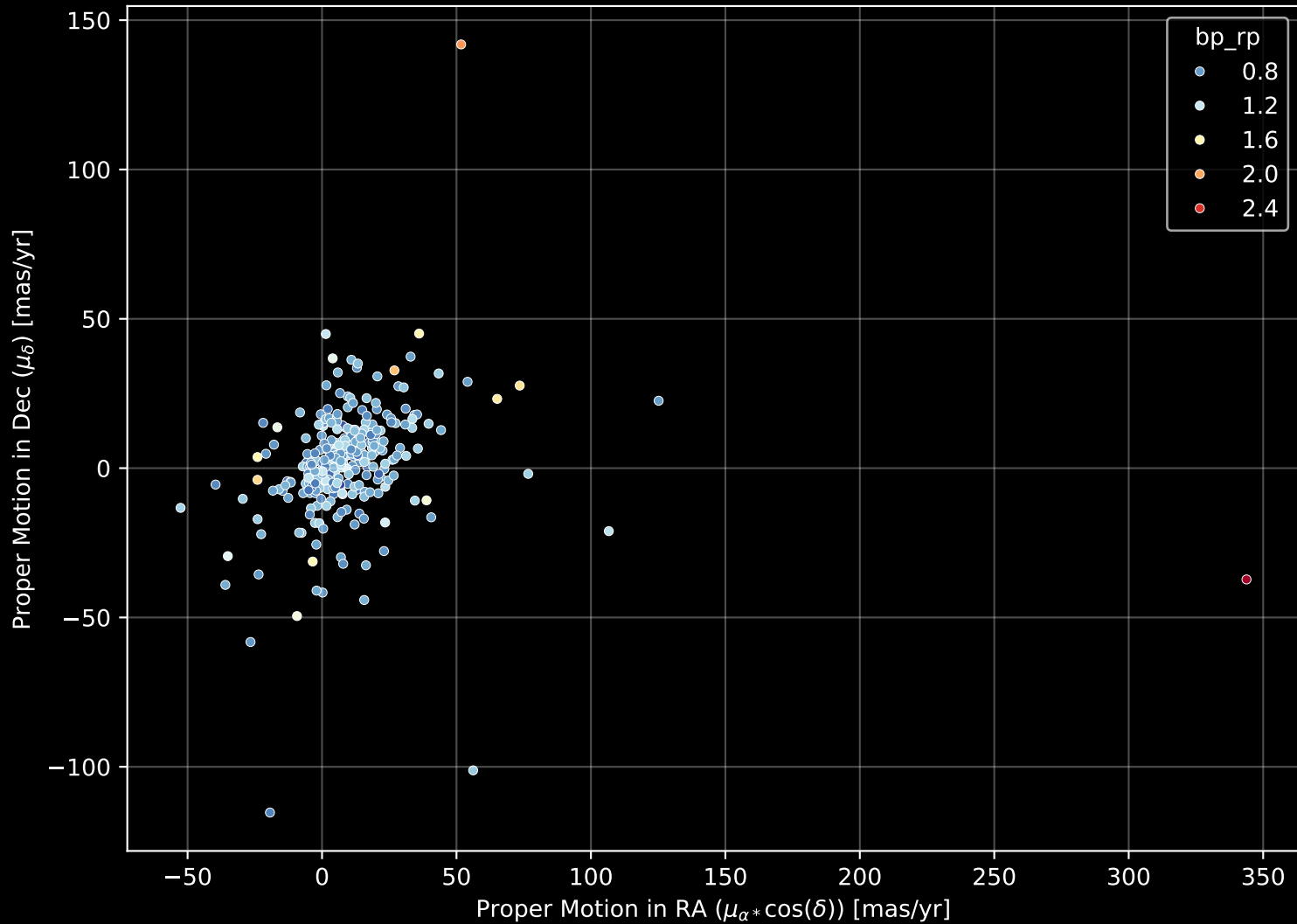
GALAH DR4 Field: [7004] Proper Motion Diagram (n= 312)
