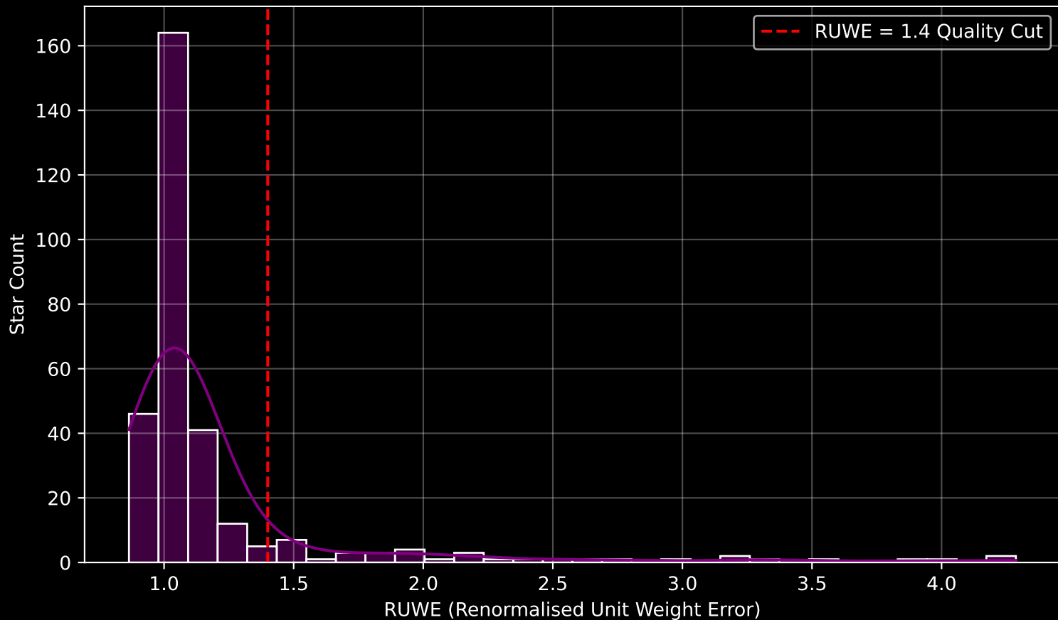
GALAH DR4 Field [7004] RUWE Distribution (n= 304)
